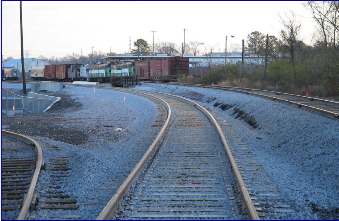
December 12, 2005 – Completed Southern Junction By-Pass Track
